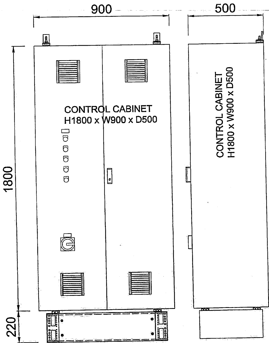
FRONT & SIDE VIEW OF CONTROLLER
